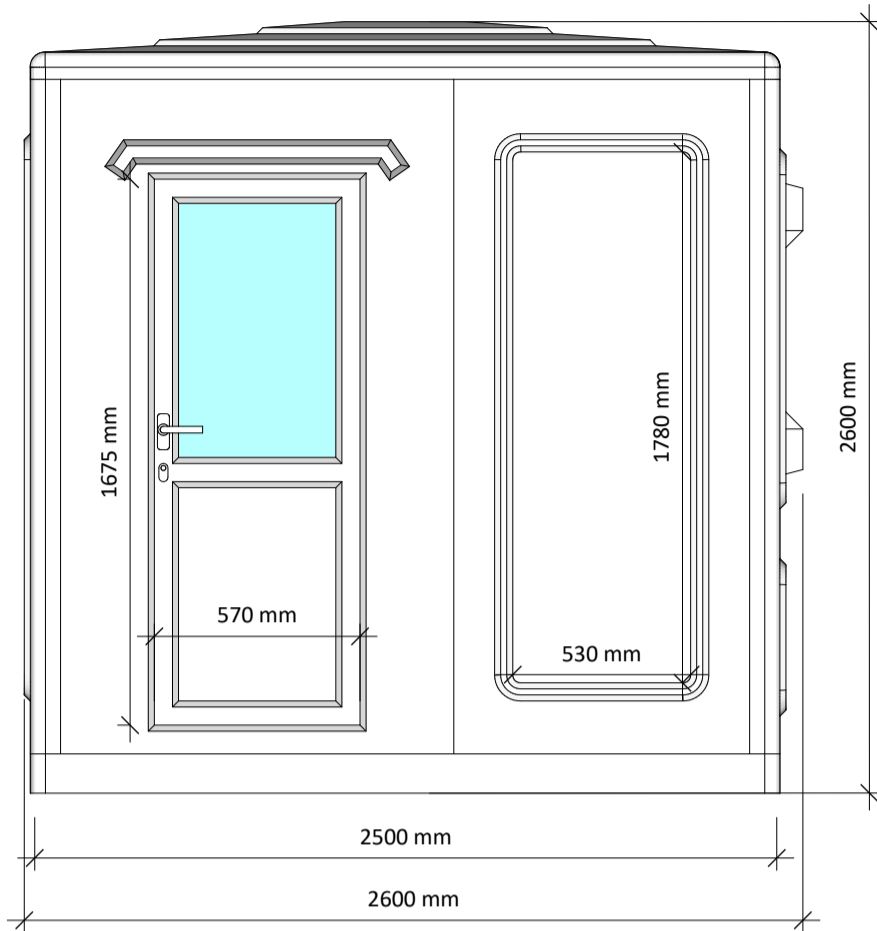
ELEVATION 'A'
