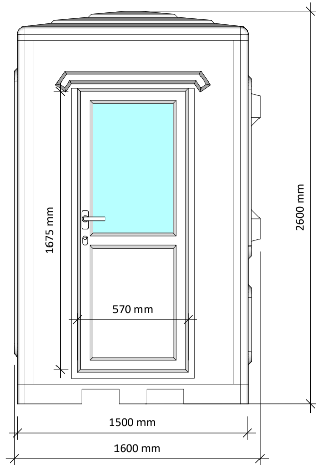
ELEVATION 'A'
